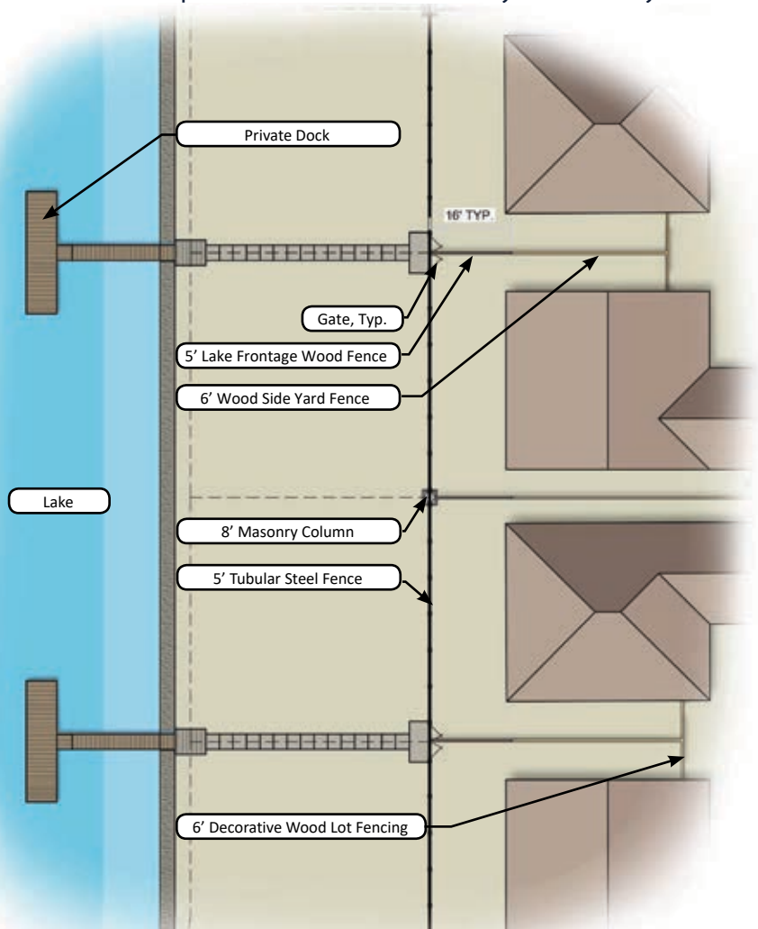
Figure 3-7: Prototypical Fence Conditions (Water Edge)
