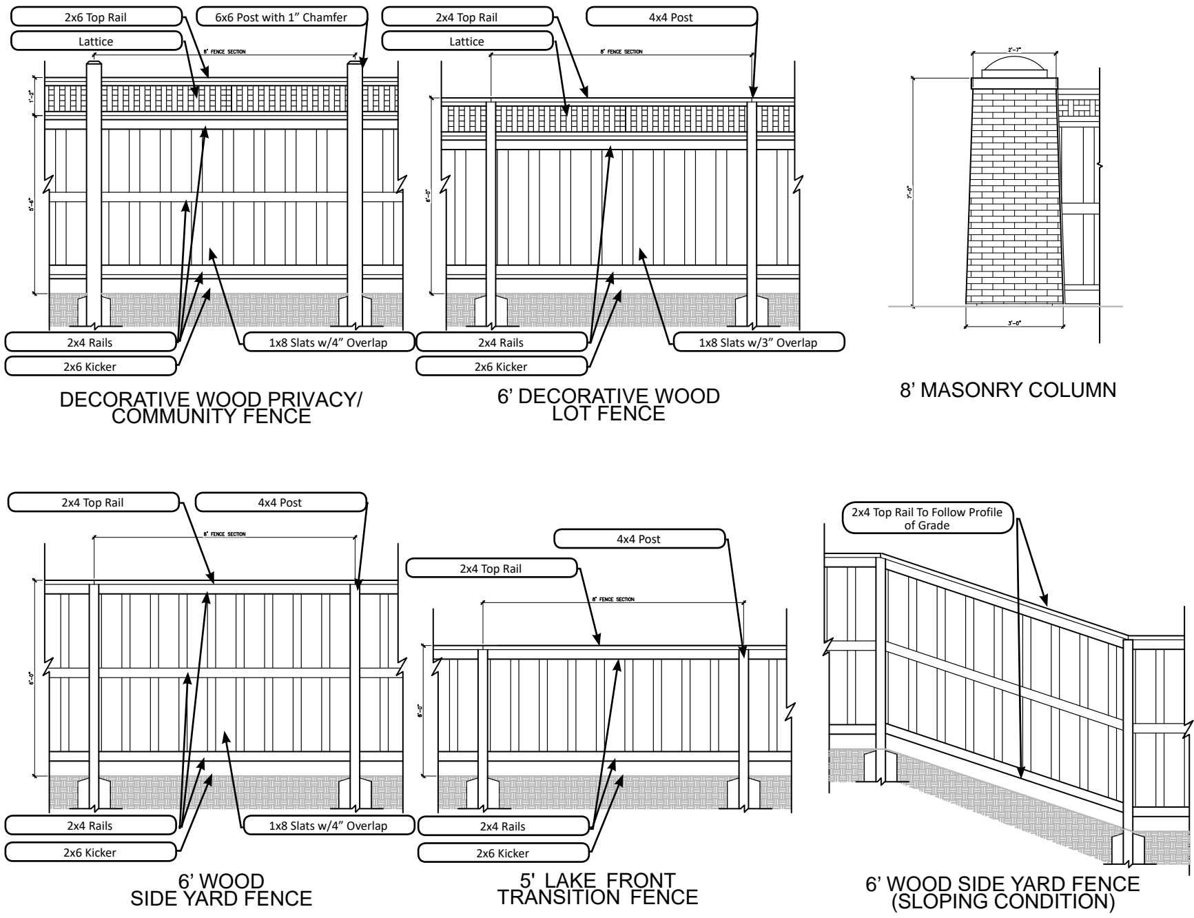
Figure 3-8: Prototypical Fence Conditions (For Builder/Developer)
