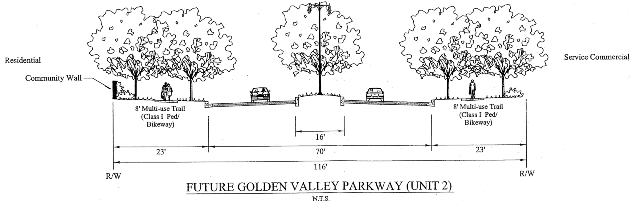
Figure 6: Street Sections – Golden Valley Parkway
