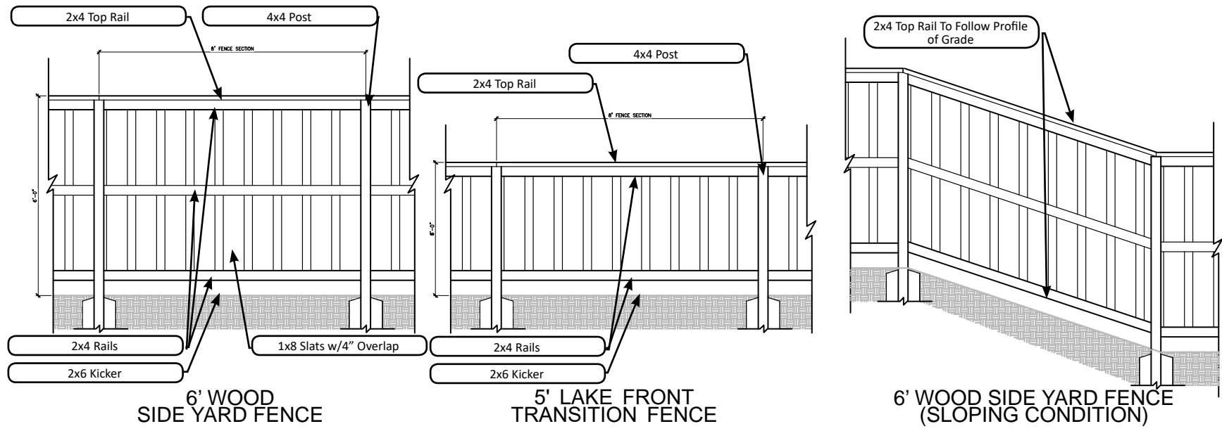
Figure 3-13: Prototypical Fence Conditions (For Builder)
