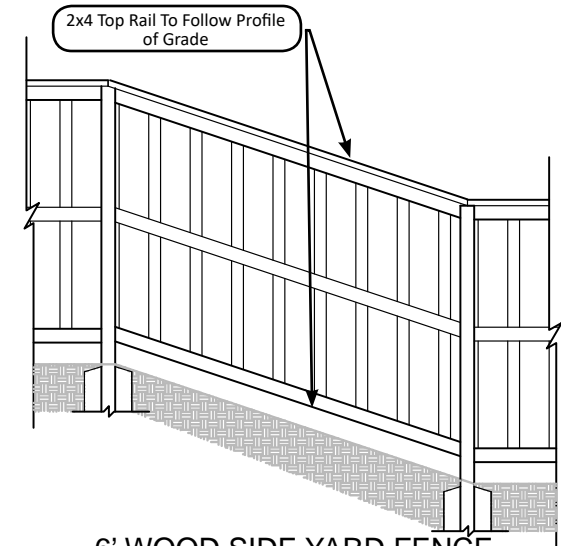
6' WOOD SIDE YARD FENCE (SLOPING CONDITION)
