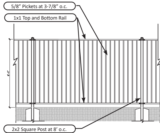
6' TUBULAR STEEL FENCE AT LAKE FRONTAGE (WHEN USED)
