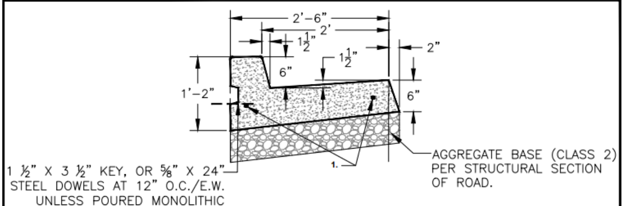
VERTICAL CURB & GUTTER
