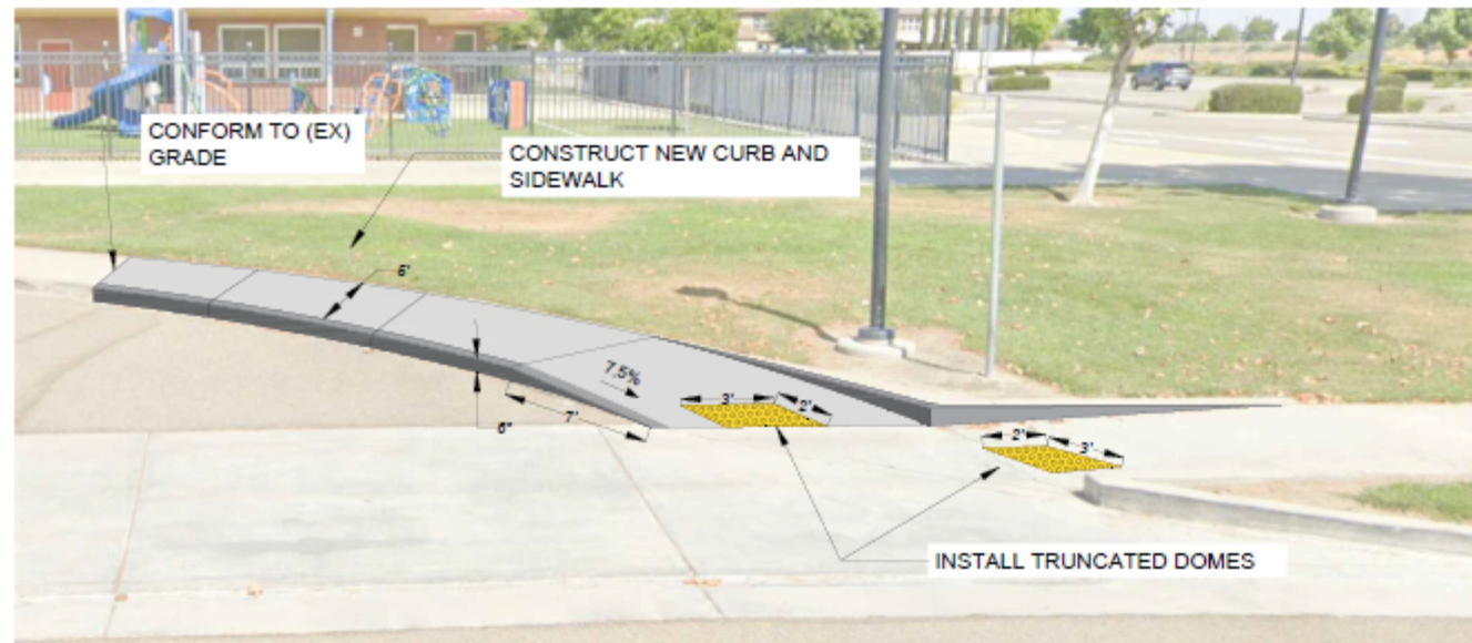
GOLDEN SPIKE TRAIL - SOUTHERLY RAMP IMPROVEMENTS (N.T.S.)
