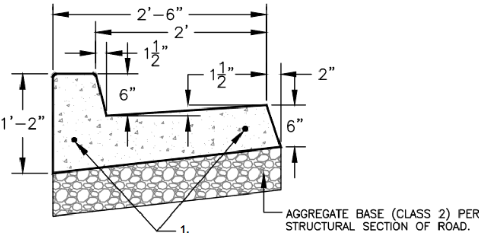
VERTICAL CURB & GUTTER
