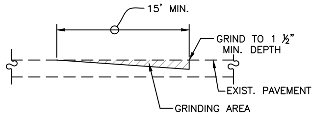
SECTION B
