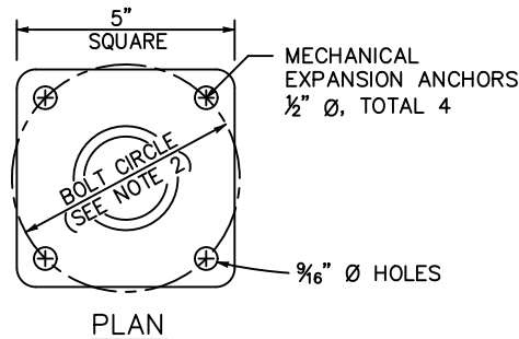
POST ANCHORAGE DETAIL
