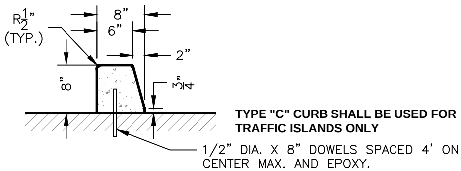
TYPE "C" CURB
