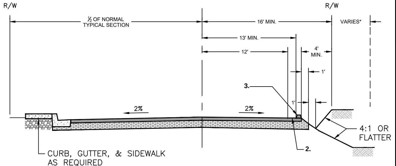
TYPICAL PARTIAL WIDTH STREET
