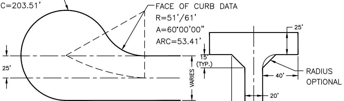
HAMMERHEAD TURNAROUND NOT TO SCALE
