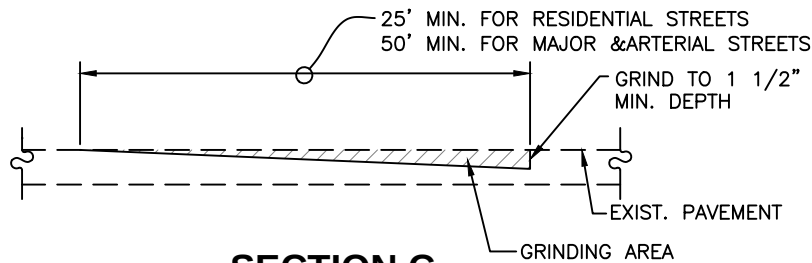
SECTION C
