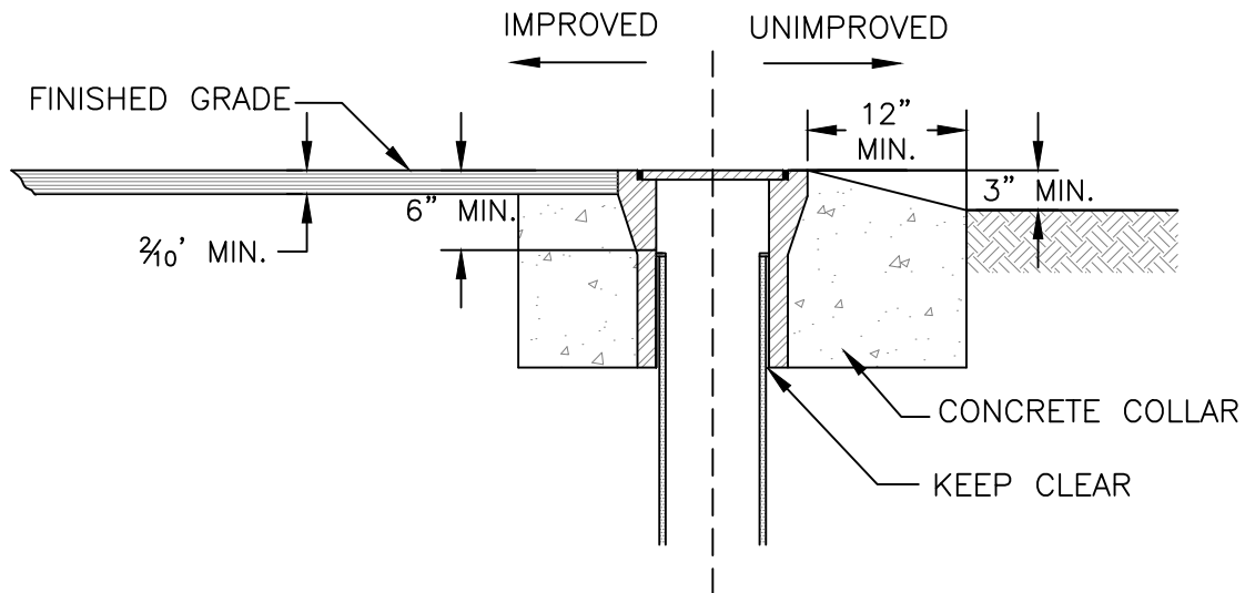
CHRISTY G5 OR G12 LID DETAIL
