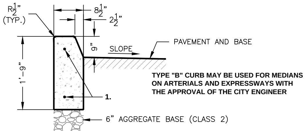
TYPE "B" VERTICAL CURB
