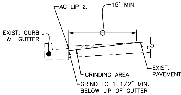
SECTION A
